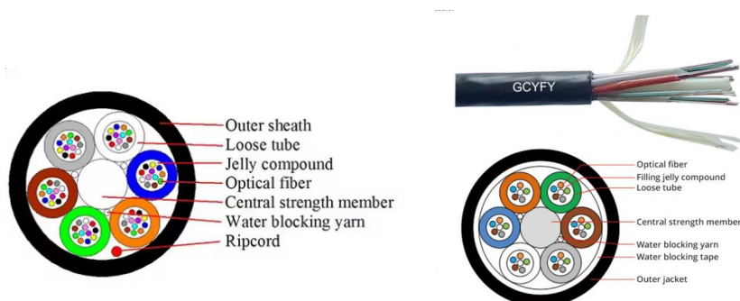
Cable structure
